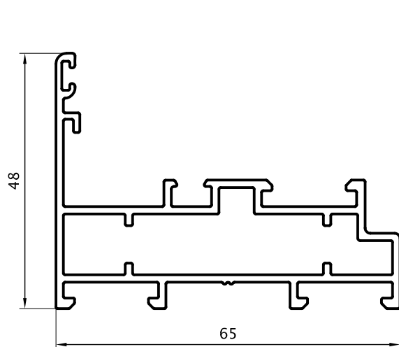
Marco Rebatir 65mm 1,000 Kg/m 08018 Barras de 6.05m
